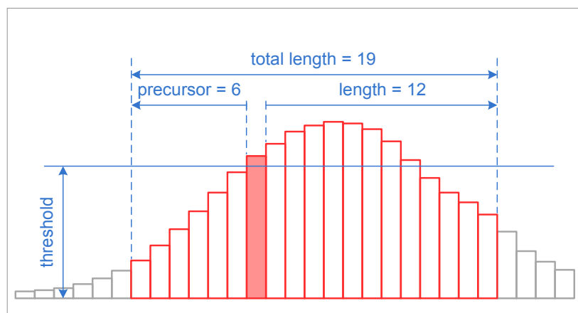
Figure 2.11: Parameters for edge triggering
